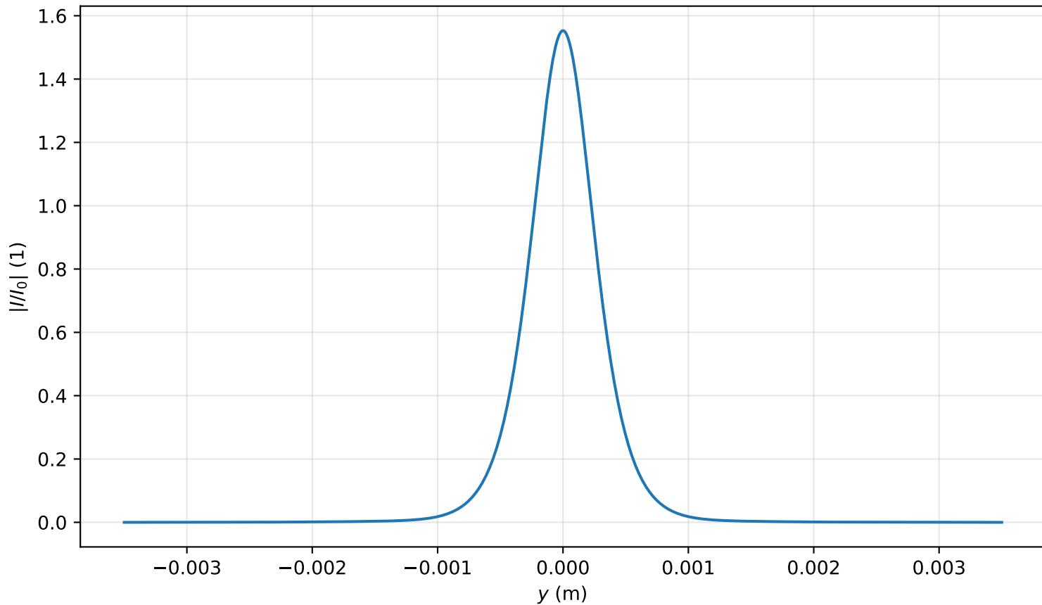
Intensity profile I(x=0, y, z=3.105)/I_0 , P_{in}=0.9P_{cr} , artificial time
